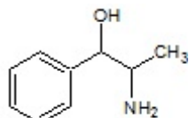
Norephedrine
